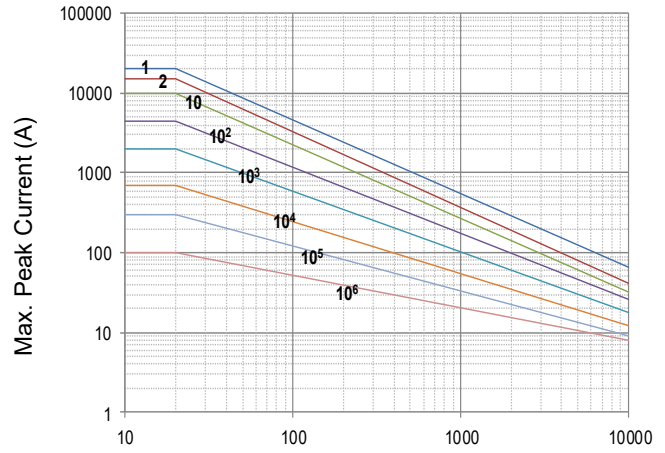
Impulse Duration (µs) SFV25D820KT to SFV25D122KT
